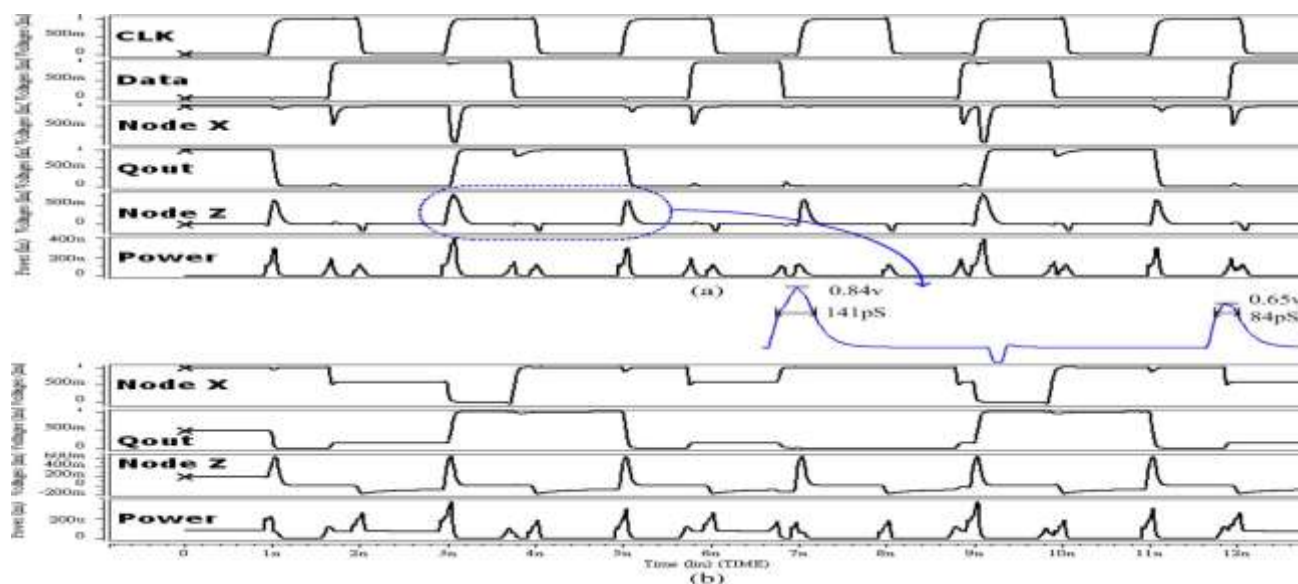
Figure 4. Simulation waveforms of (a) proposed and (b) MHLFF designs. Feature Comparison Of Various P-Ff Designs
