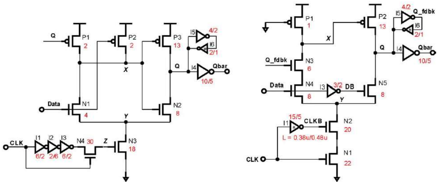
Figure 1. Conventional pulse-triggered FF designs (a) MHLFF (b) SOCCER.
