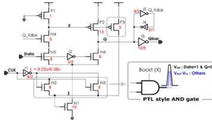
Figure 2. Schematic diagram of the proposed P-FF design with pulse enhancement scheme.
